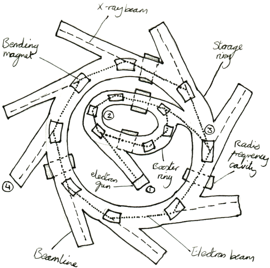
22/03/13 - DIAGRAM OF A SYNCHROTRON FR
